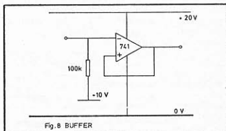
Fig. 8 BUFFER
